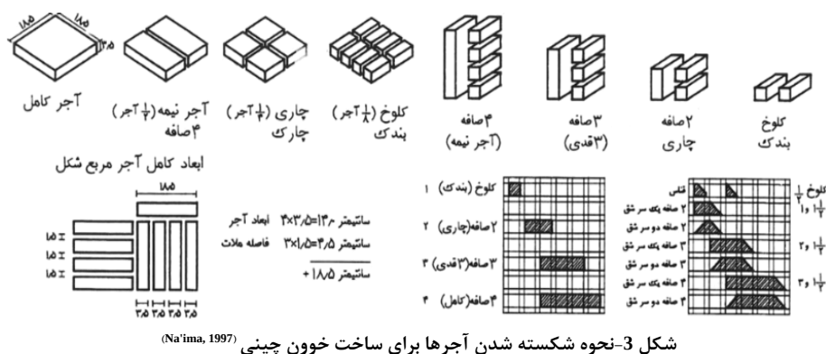
Fig. 3-The method of brick fracturing for Khoon-Chini construction (Na'ima, 1997)
